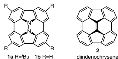
Figure 1. Hydrazinobuckybowls 1 and diindenochrysene ( 2 ).
